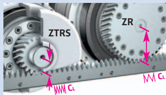
Linear stiffness through small lever arm.
